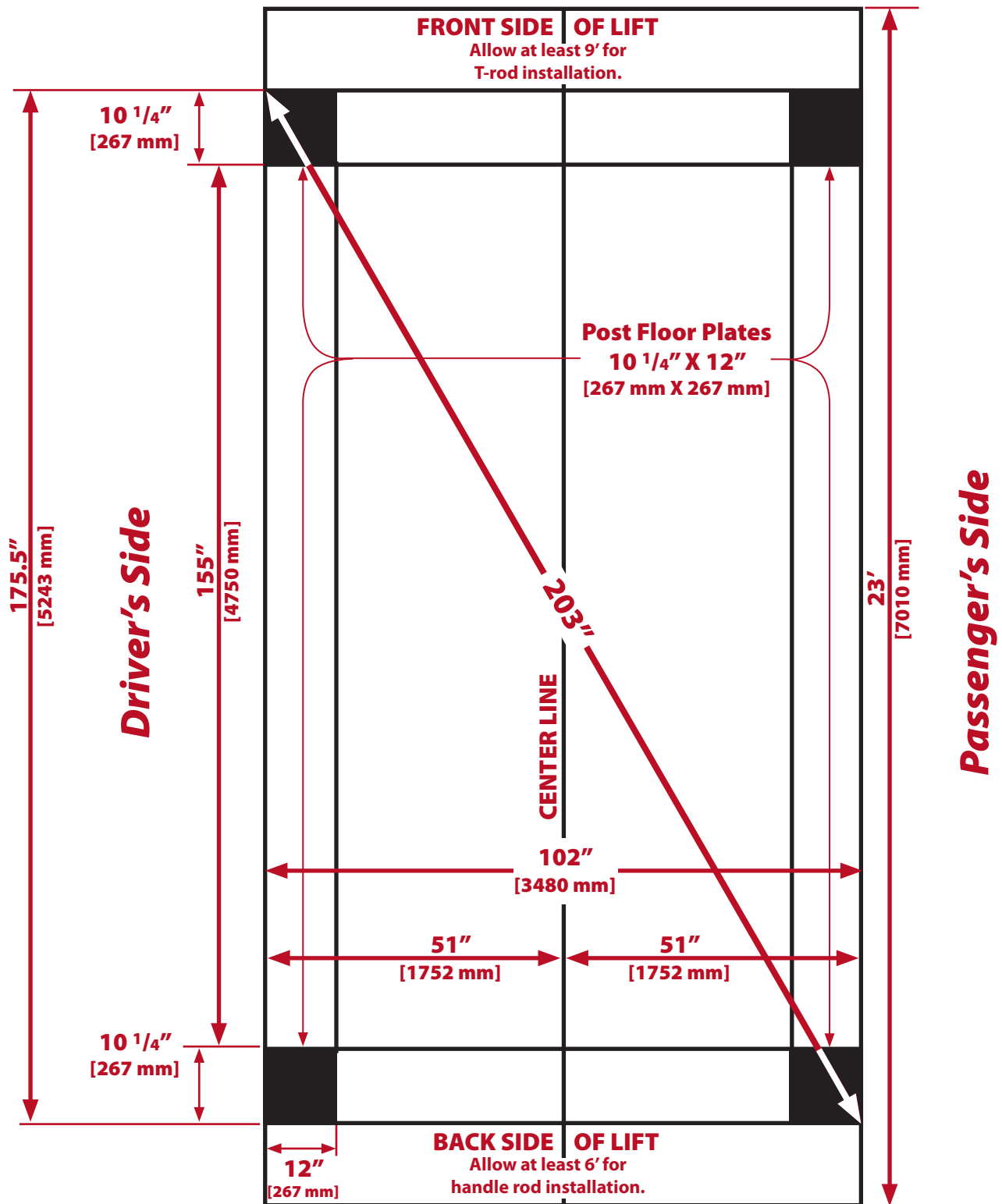
FIGURE 2a (CL 8,000 CSP Layout Drawing)
