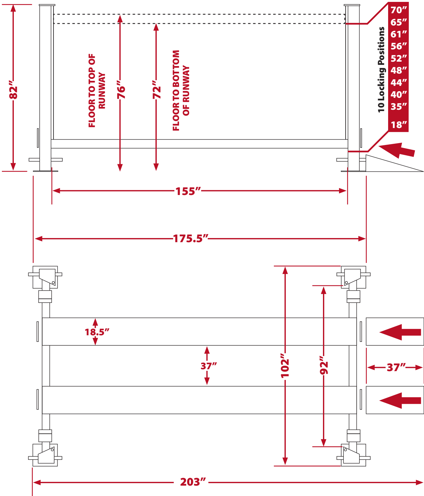
FIGURE 1a (CL 8,000 CSP Specifications Drawing)
