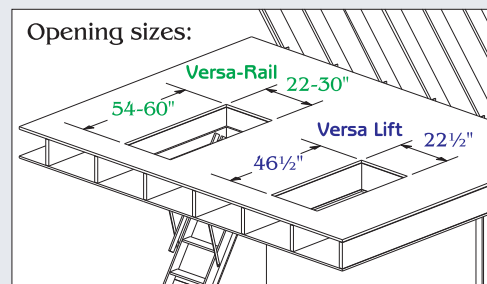
Versa Lift automatically closes the ceiling port.
